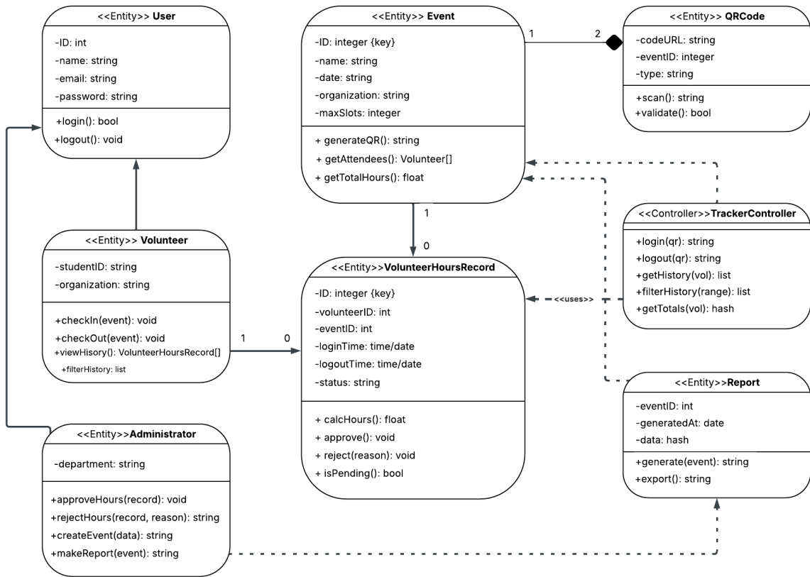
Class Diagram
